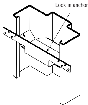
Anchor for Stud Partition
