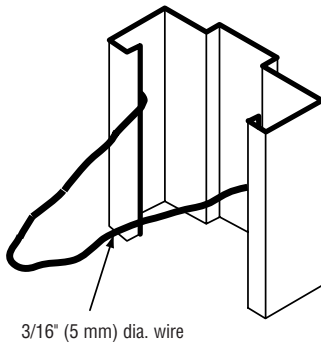
Wire Masonry Anchor
