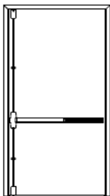
Figure 11.5: WS98/9927 2-point latch (shown) WS98/9957 (not shown) is similar but is a 3-point latch, adding a center latch point.
