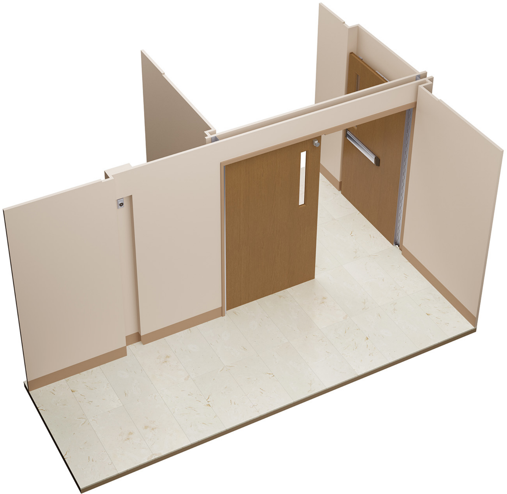
INPACT SYSTEM SET D4 (700 stainless pin & barrel continuous hinge on door opening 90 degrees and 040XY alum wide throw continuous hinge on door opening 180 degrees)
